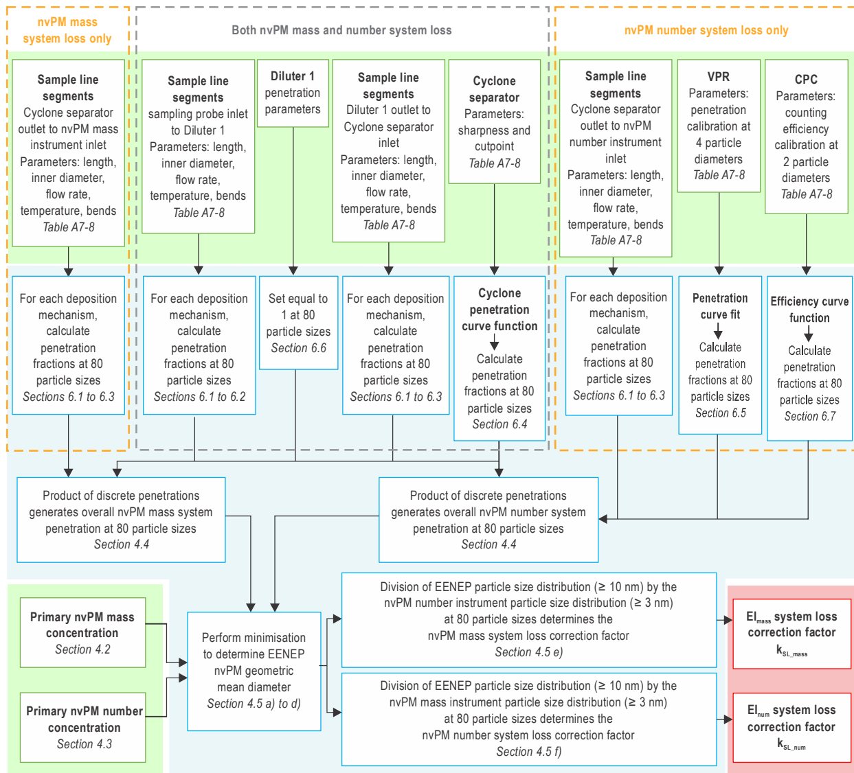
Figure A8-1. Flow block diagram of the nvPM system loss correction methodology. The green blocks show model input parameters, the blue blocks shows model calculations and the red outline blocks shows calculation output system loss correction factors.
