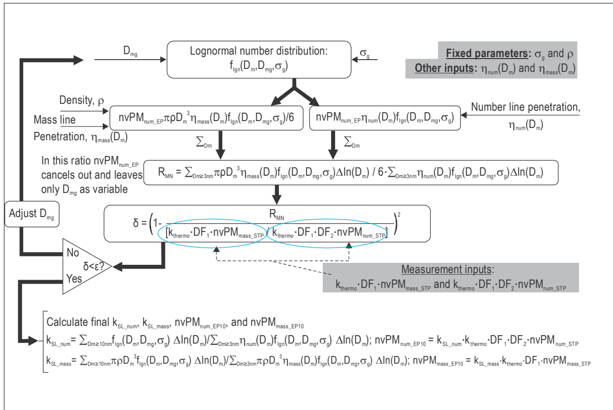
Figure A8-2. Iterative calculation procedure diagram for determination of system loss correction factors
